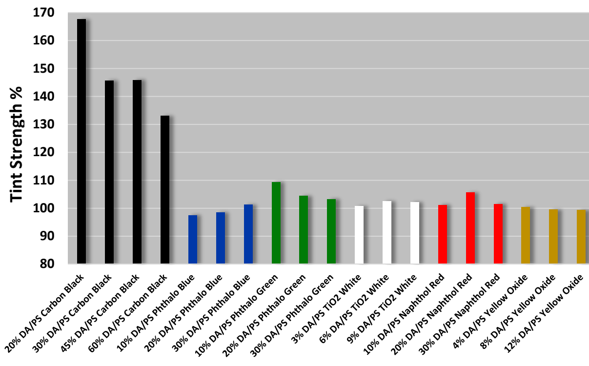
Tint strength of SURFONIC® 3620 Dispersant versus a commercial standard at the same level of dispersant actives on pigment solids (DA/PS)
